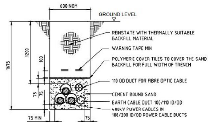
GENERAL INSTALLATION
