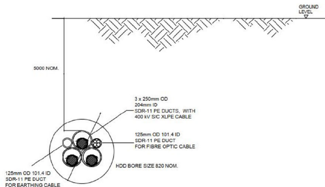
HDD INSTALLATION
